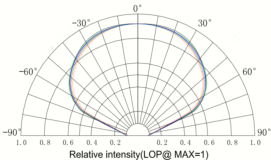
Beam Pattern
